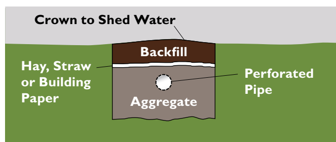
Figure 3: Cross-sectional view through trench
