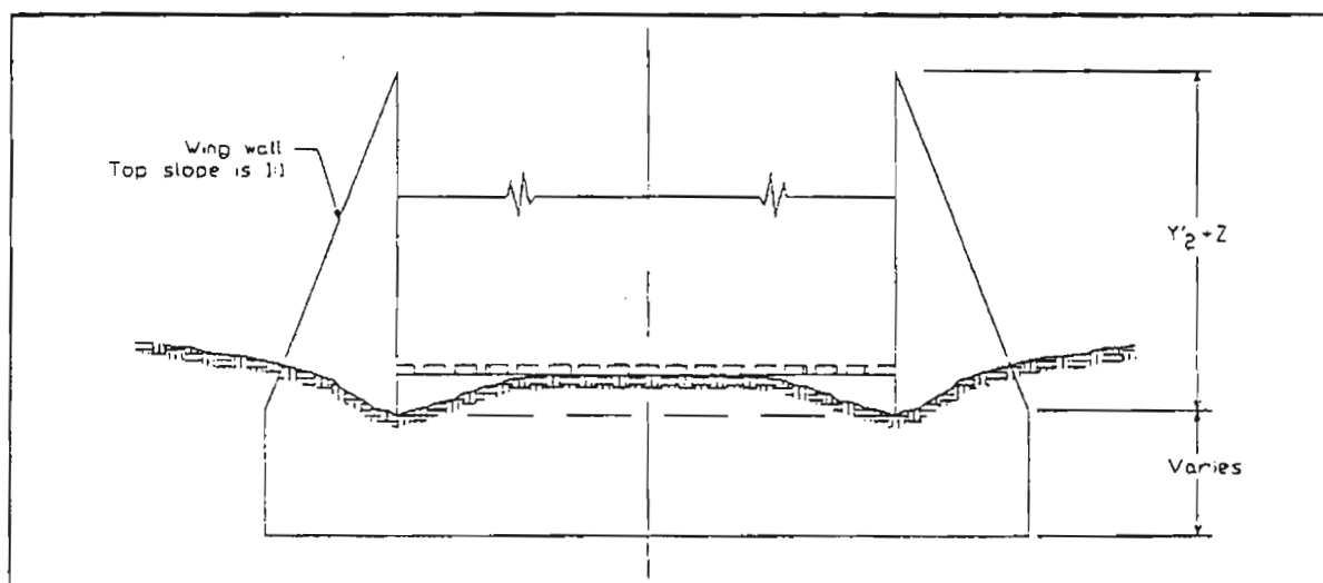
FIGURE 6.12 Downstream Elevation of Rectangular SAF-Type Stilling Basin
