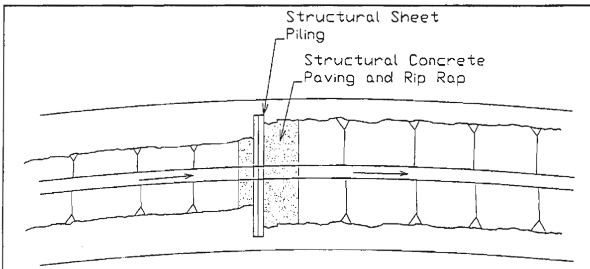
FIGURE 6.4 Plan View of Typical Straight Drop Spillway
