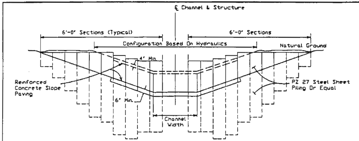
FIGURE 6.3 Cross-Section of Typical Straight Drop Spillway
