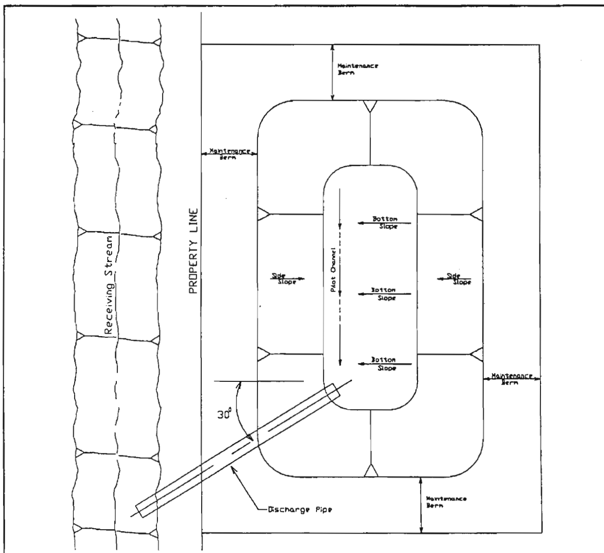
FIGURE 7.2 Typical Detention Basin Configuration
