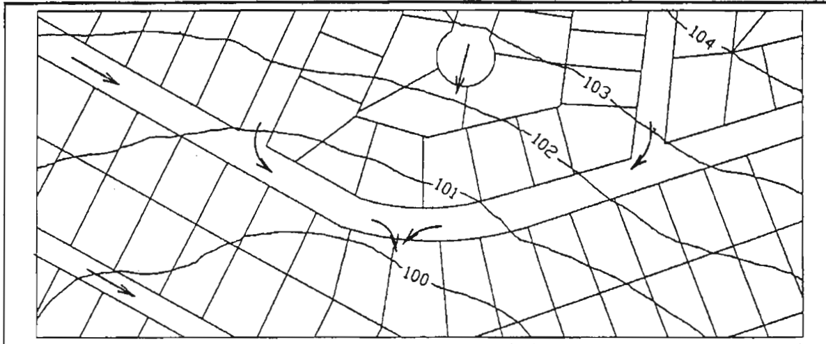
FIGURE 5.9 Undesirable Overland Flow Pattern at Roadway Curve
