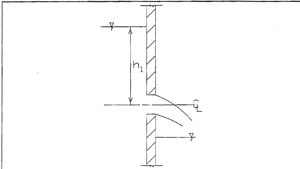
FIGURE 7.13 Unsubmerged Orifice
