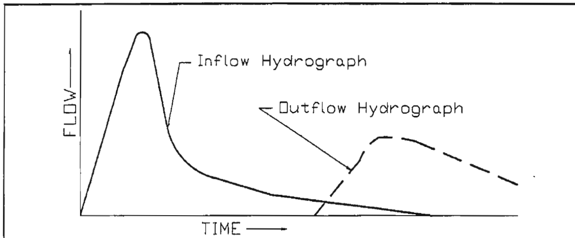
FIGURE 7.3 Effect of Retention Storage on Hydrographs
