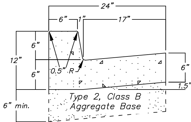
TYPE 1 CURB & GUTTER
