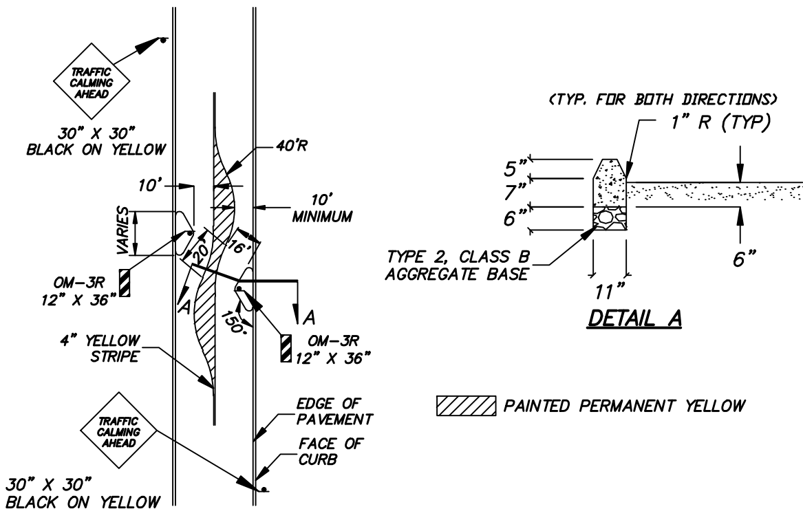
PLAN - STRIPING AND SIGNAGE
