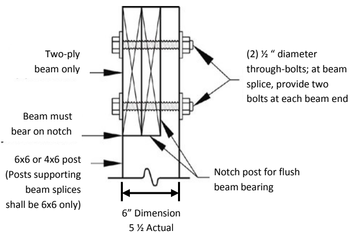
Notched Post
