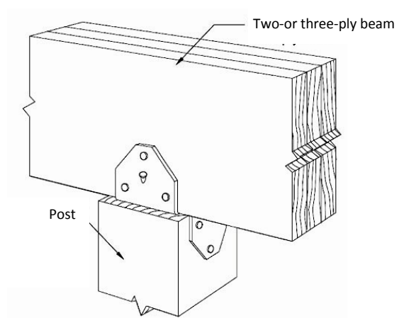
Post Cap
